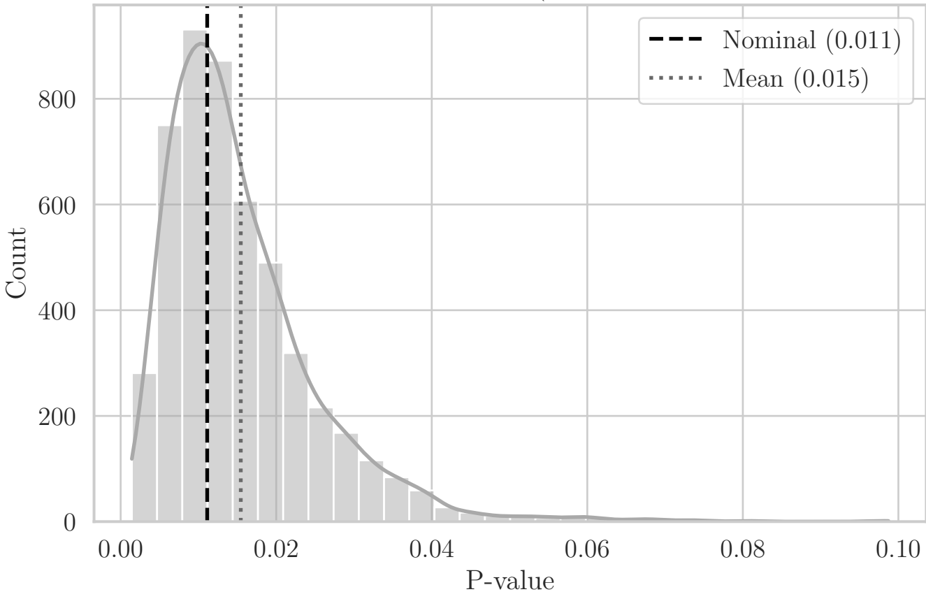
MC Distribution of P-values for T Distance (Aggregated Bottom-Left Quadrant YZ)
