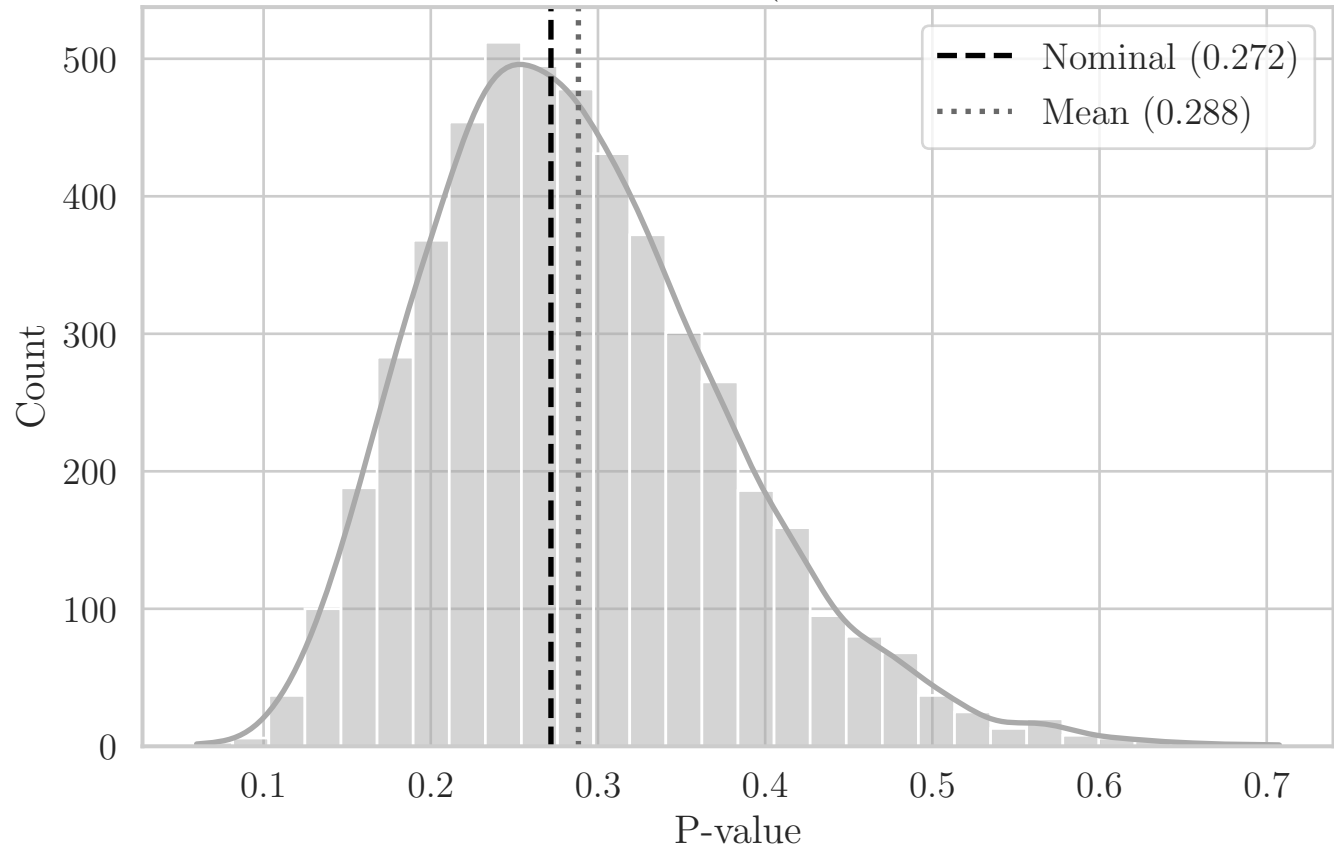
MC Distribution of P-values for T Solidity (Aggregated Bottom-Left Quadrant YZ)
