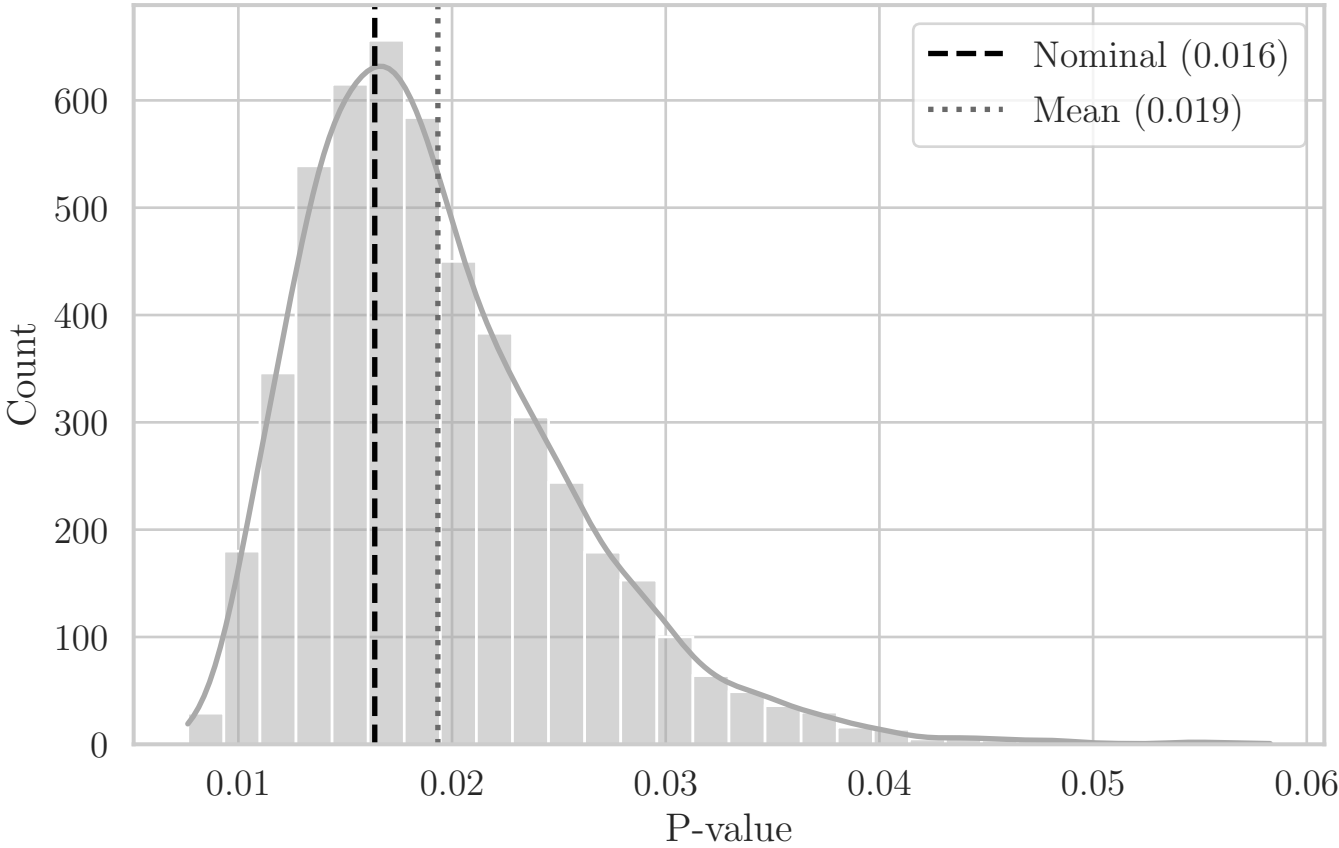
MC Distribution of P-values for QRS Area_Net (Aggregated Bottom-Right Quadrant XY)
