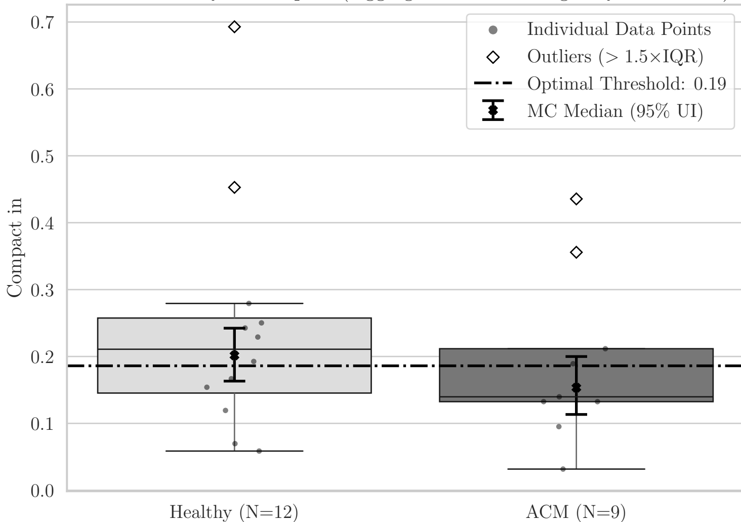
Box Plot for QRS Compact (Aggregated Bottom-Right Quadrant XY)
