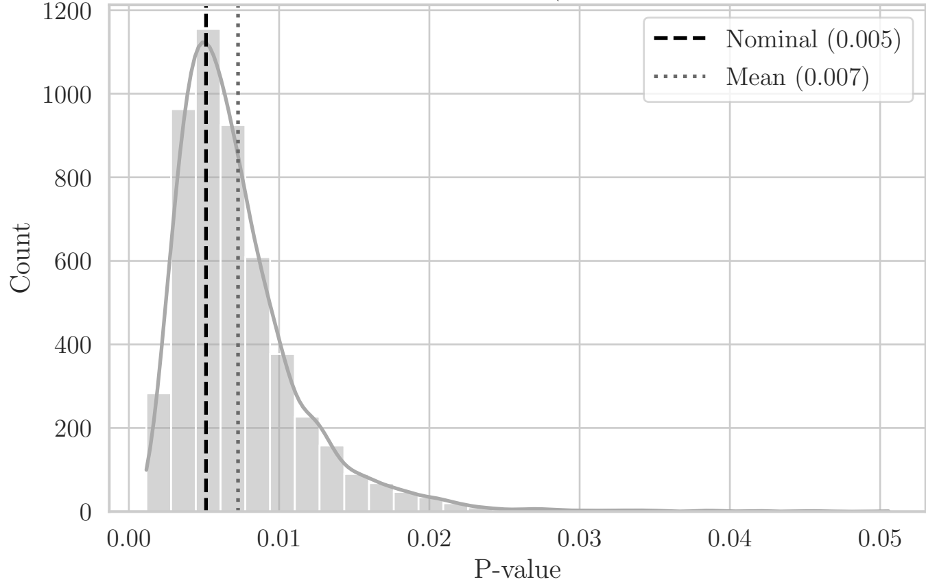
MC Distribution of P-values for QRS Distance (Aggregated Bottom-Right Quadrant XY)
