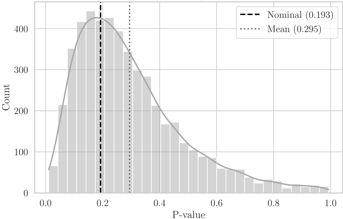
MC Distribution of P-values for QRS Solidity (Aggregated Bottom-Right Quadrant XY)
