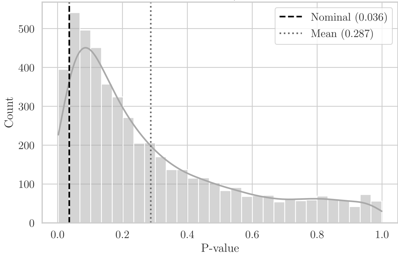
MC Distribution of P-values for ST Area_Net (Aggregated Bottom-Right Quadrant XY)
