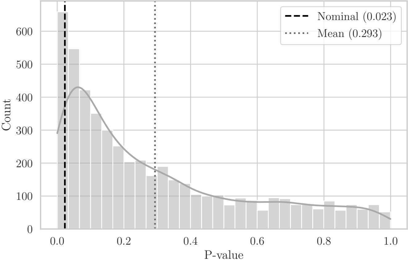
MC Distribution of P-values for ST Distance (Aggregated Bottom-Right Quadrant XY)
