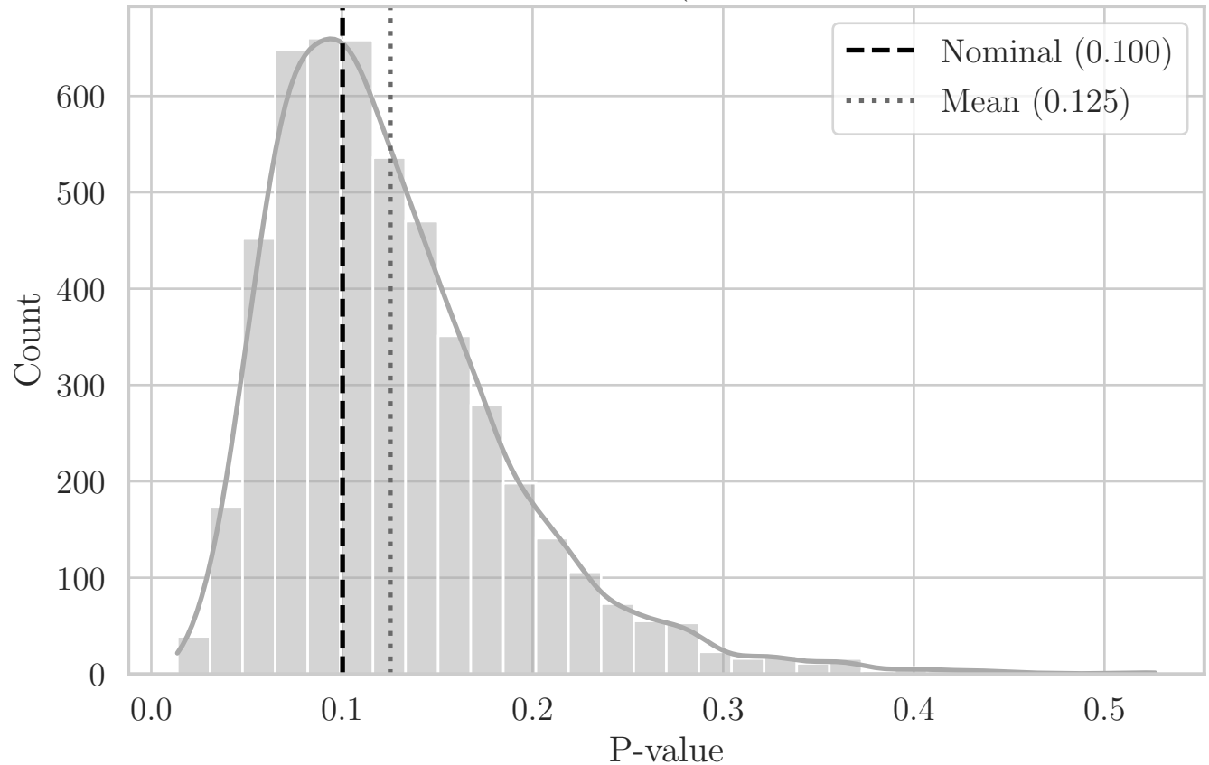
MC Distribution of P-values for T Solidity (Aggregated Bottom-Right Quadrant XY)
