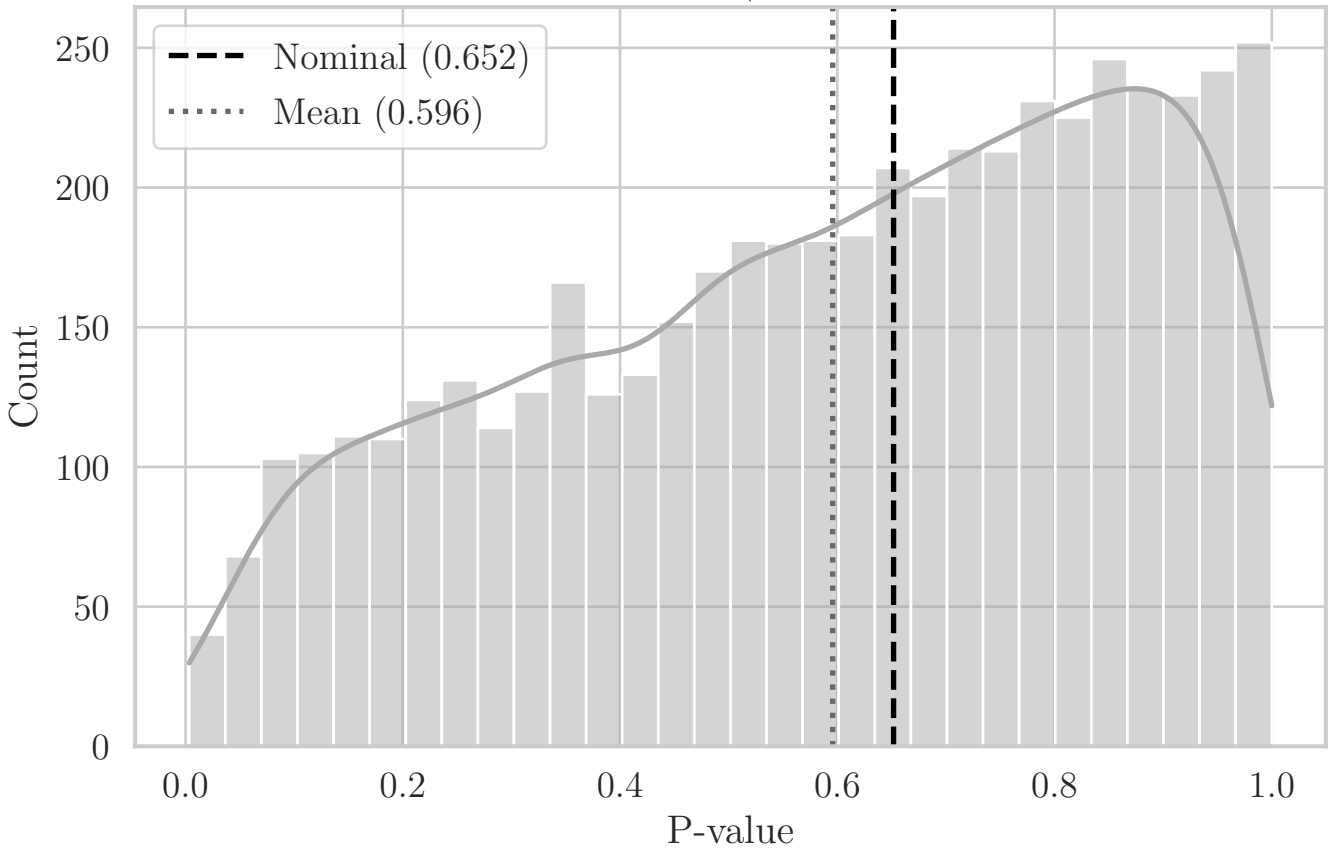
MC Distribution of P-values for ST Angle (Aggregated Bottom-Right Quadrant YZ)
