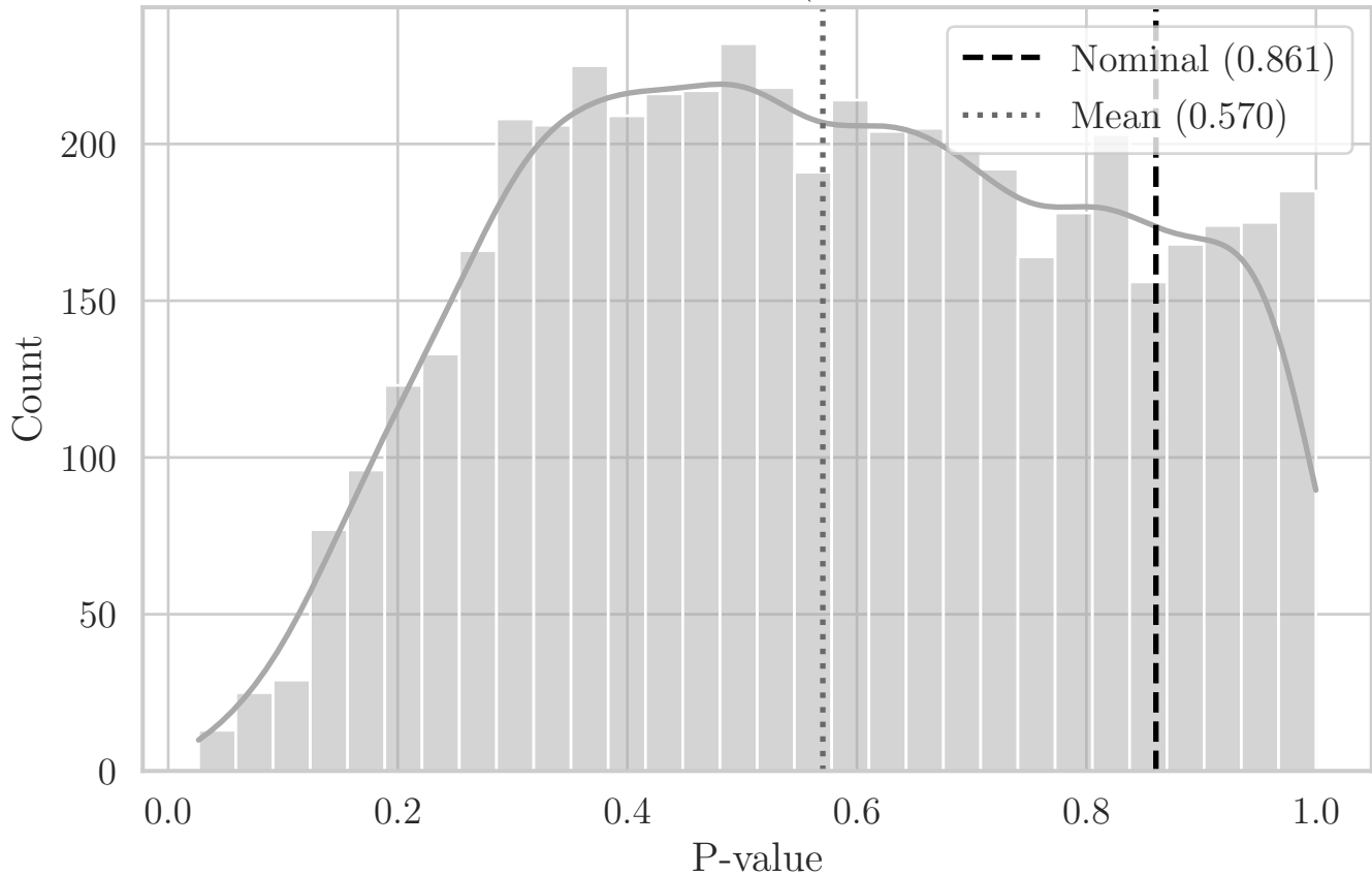
MC Distribution of P-values for ST Area_Net (Aggregated Bottom-Right Quadrant YZ)
