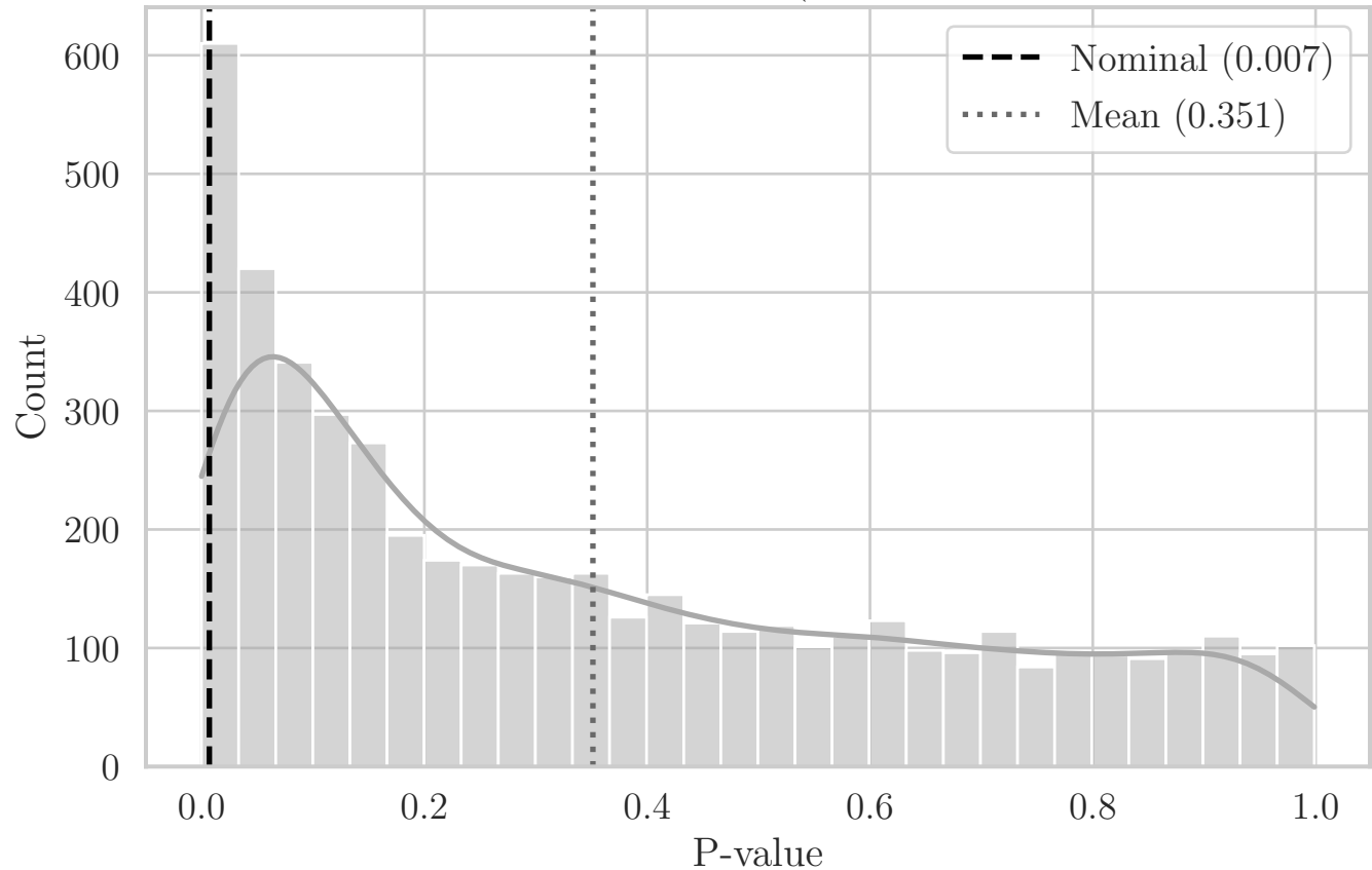
MC Distribution of P-values for ST Distance (Aggregated Bottom-Right Quadrant YZ)
