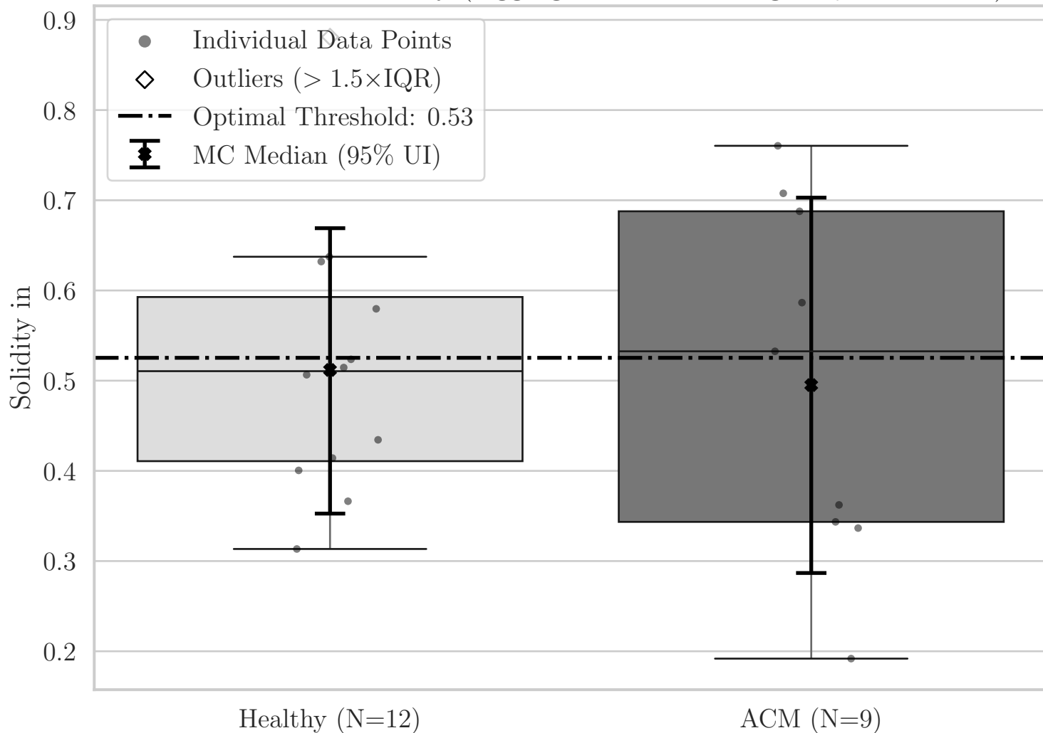
Box Plot for ST Solidity (Aggregated Bottom-Right Quadrant YZ)
