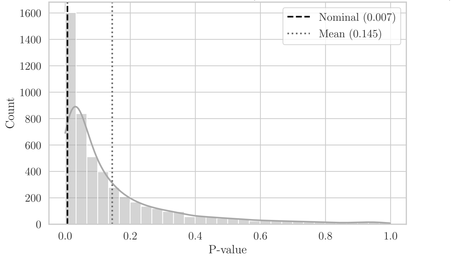
MC Distribution of P-values for ST Distance (Aggregated Top-Left Quadrant XY)
