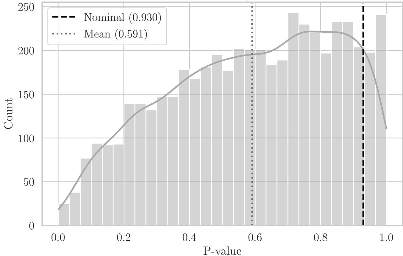
MC Distribution of P-values for ST Solidity (Aggregated Top-Left Quadrant XY)
