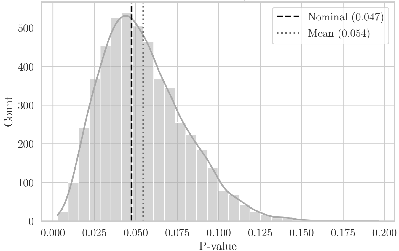
MC Distribution of P-values for T Area_Hull (Aggregated Top-Left Quadrant XY)
