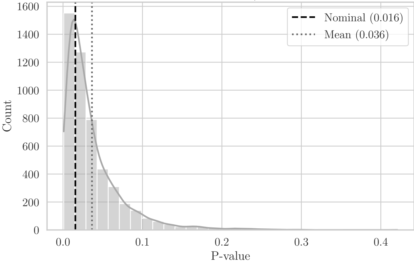
MC Distribution of P-values for T Distance (Aggregated Top-Left Quadrant XY)
