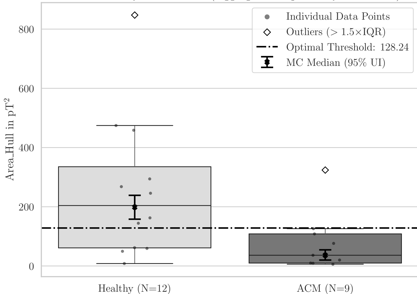
Box Plot for QRS Area_Hull (Aggregated Top-Left Quadrant YZ)
