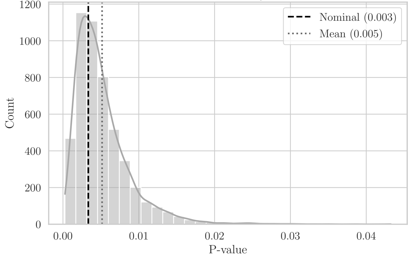
MC Distribution of P-values for QRS Distance (Aggregated Top-Left Quadrant YZ)
