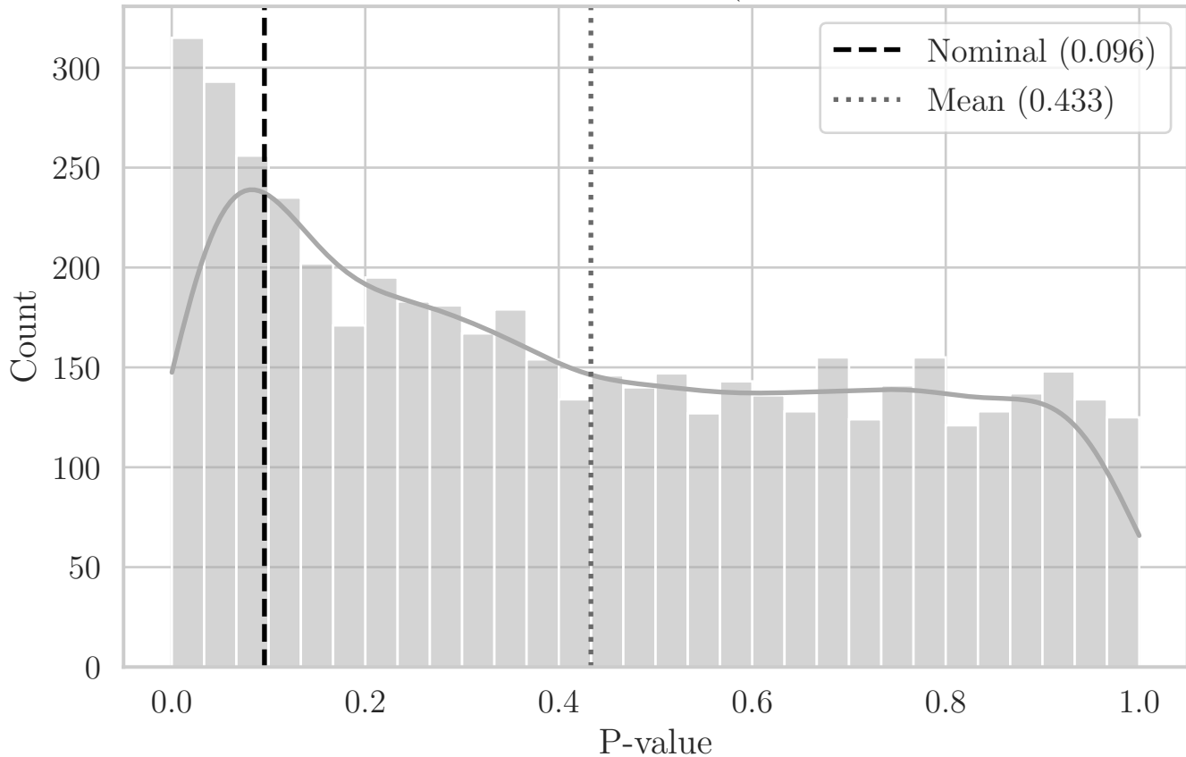
MC Distribution of P-values for ST Distance (Aggregated Top-Left Quadrant YZ)
