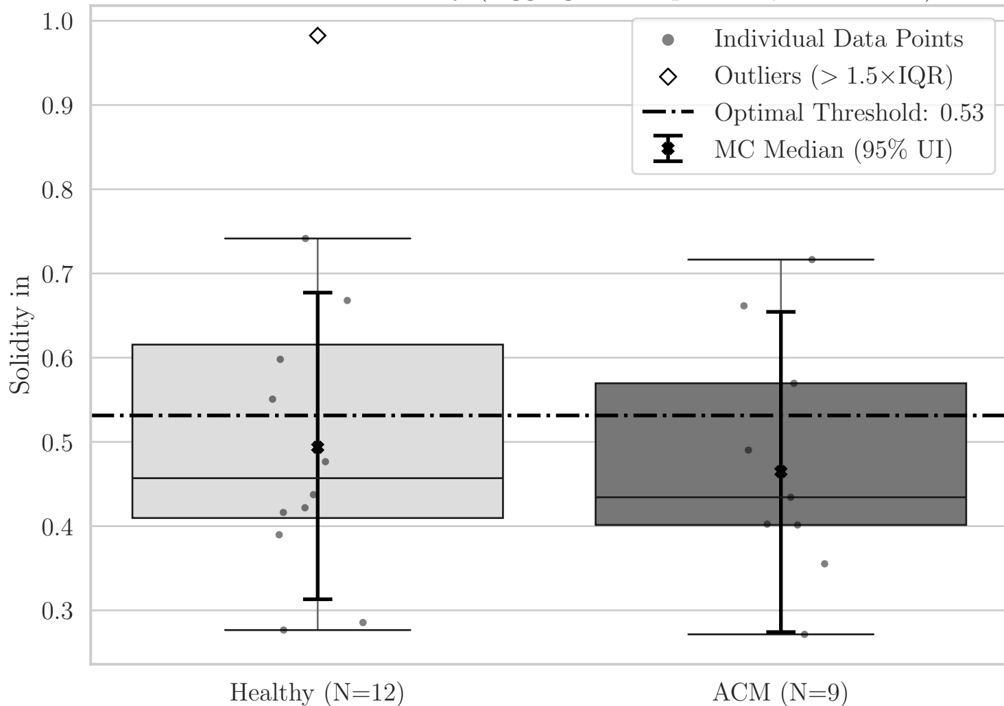
Box Plot for ST Solidity (Aggregated Top-Left Quadrant YZ)
