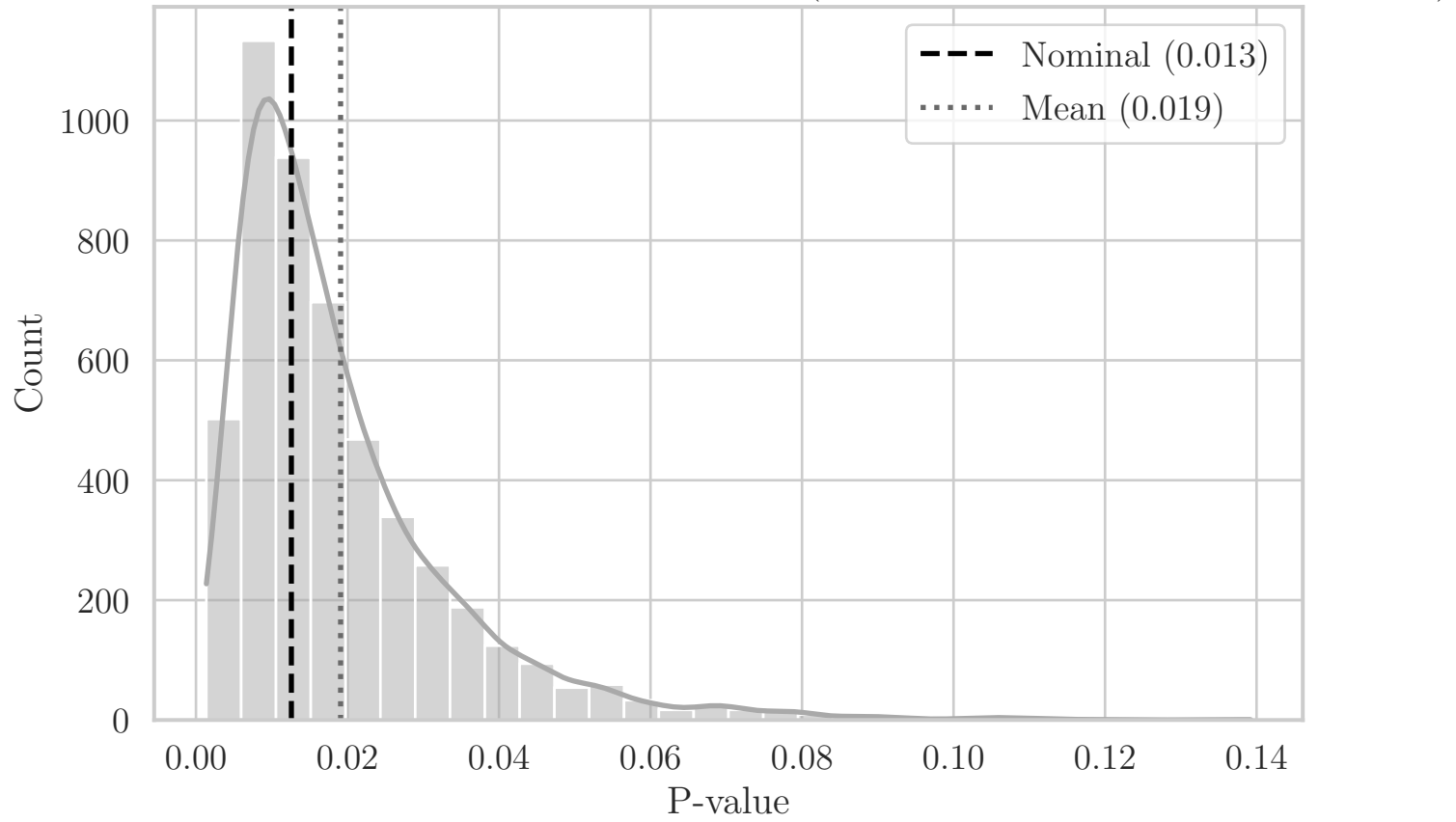
MC Distribution of P-values for T Area_Hull (Aggregated Top-Left Quadrant YZ)
