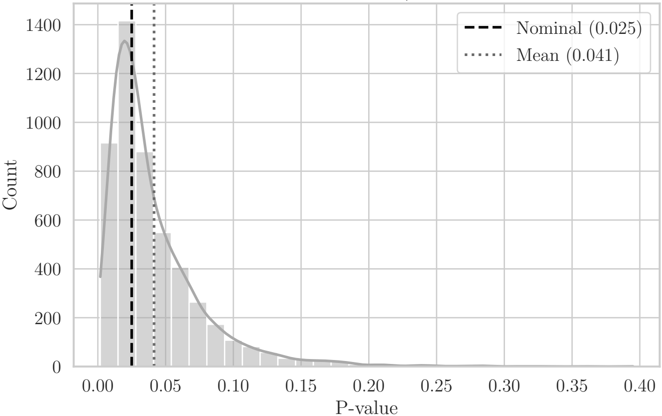
MC Distribution of P-values for T Distance (Aggregated Top-Left Quadrant YZ)
