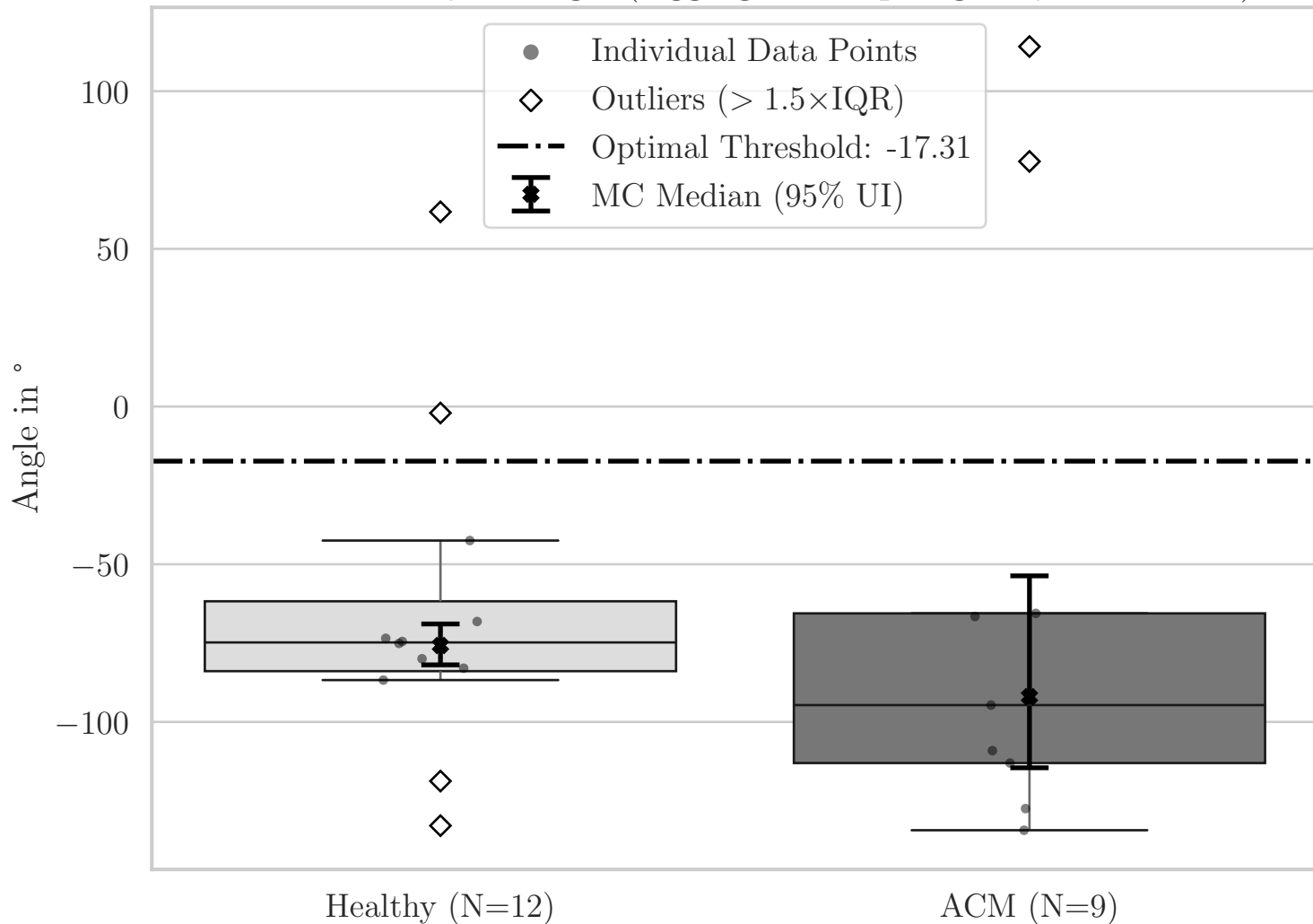
Box Plot for QRS Angle (Aggregated Top-Right Quadrant XY)
