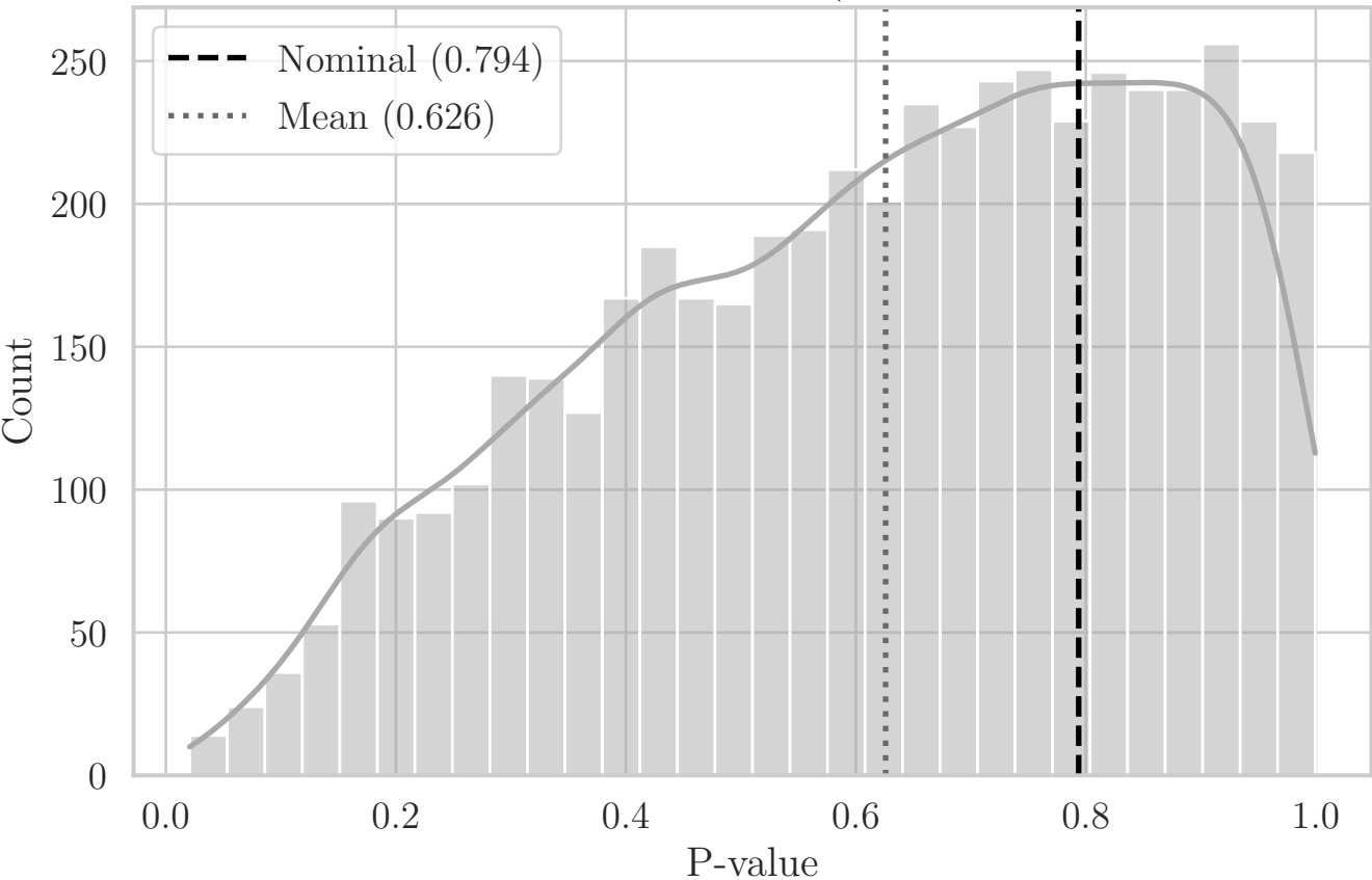
MC Distribution of P-values for QRS Solidity (Aggregated Top-Right Quadrant XY)
