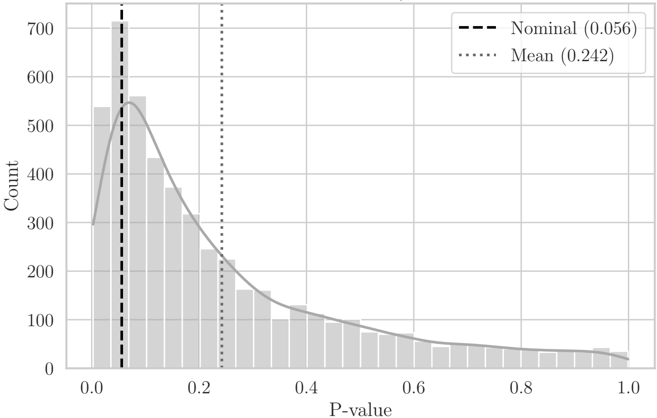
MC Distribution of P-values for ST Area_Net (Aggregated Top-Right Quadrant XY)
