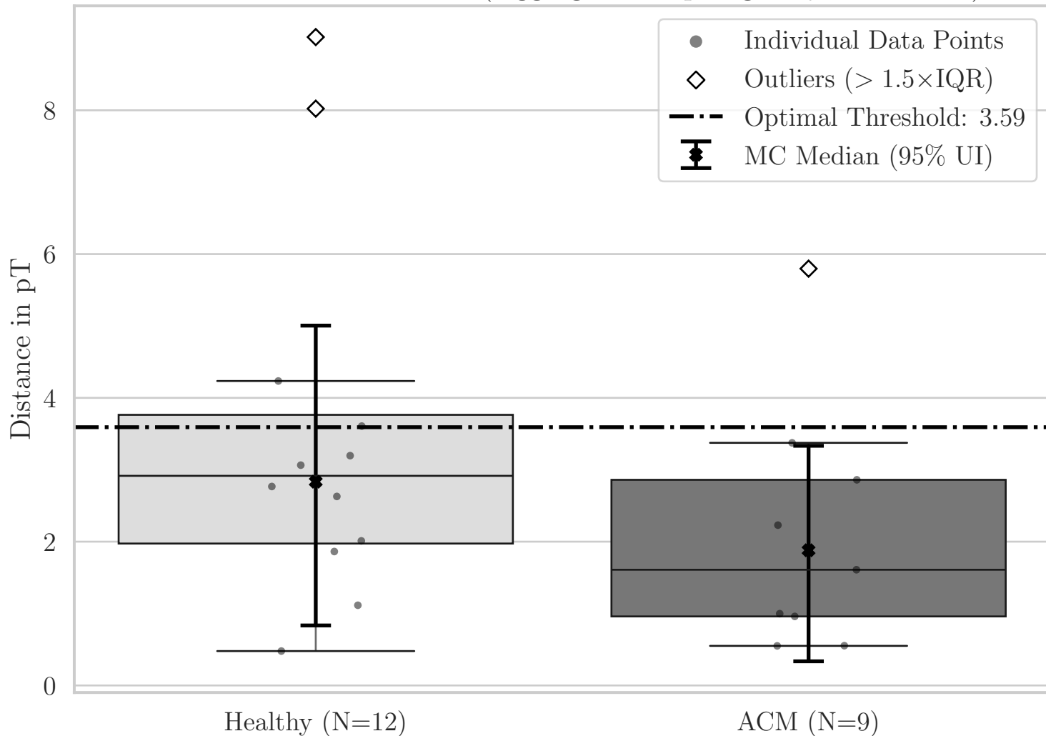
Box Plot for ST Distance (Aggregated Top-Right Quadrant XY)
