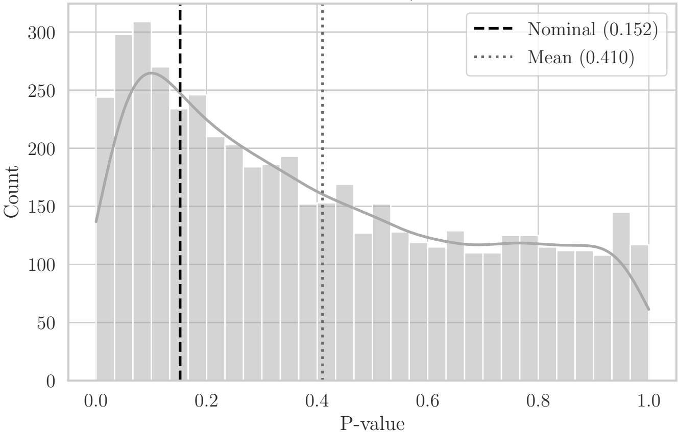
MC Distribution of P-values for ST Distance (Aggregated Top-Right Quadrant XY)
