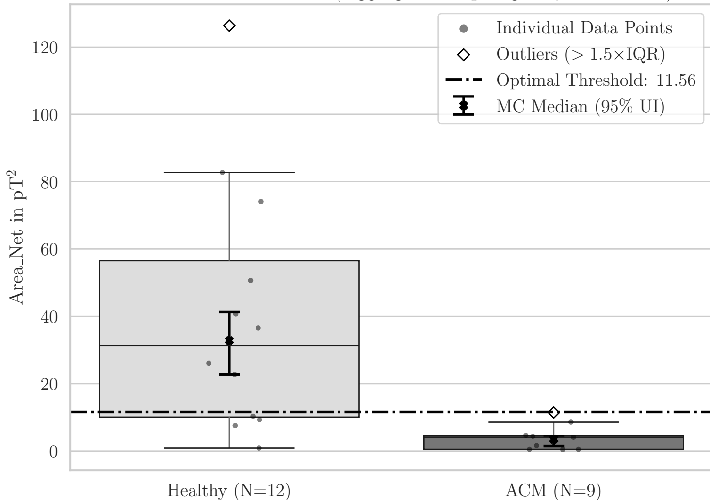
Box Plot for T Area_Net (Aggregated Top-Right Quadrant XY)
