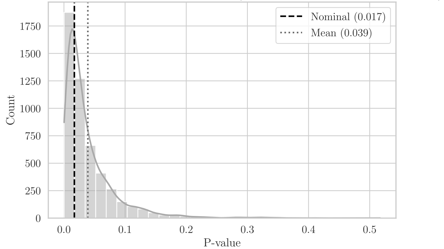
MC Distribution of P-values for T Distance (Aggregated Top-Right Quadrant XY)
