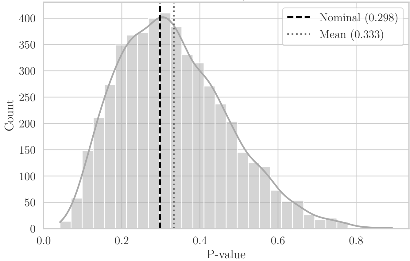
MC Distribution of P-values for T Solidity (Aggregated Top-Right Quadrant XY)
