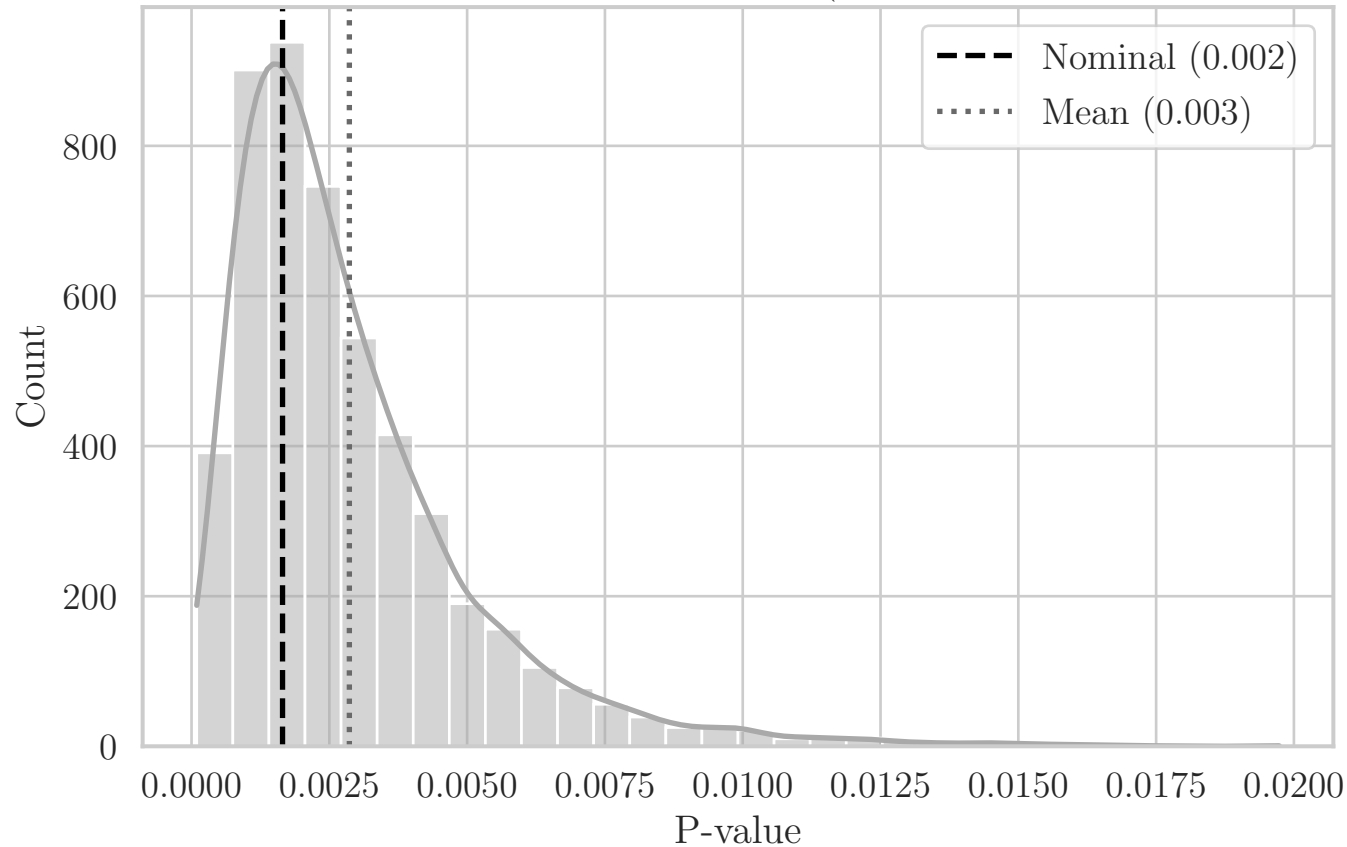
MC Distribution of P-values for QRS Distance (Aggregated Top-Right Quadrant YZ)
