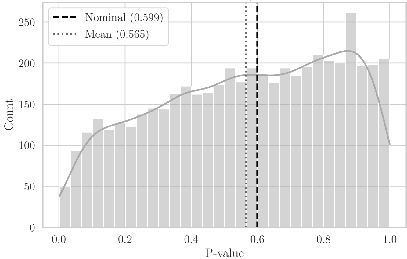
MC Distribution of P-values for ST Area_Net (Aggregated Top-Right Quadrant YZ)
