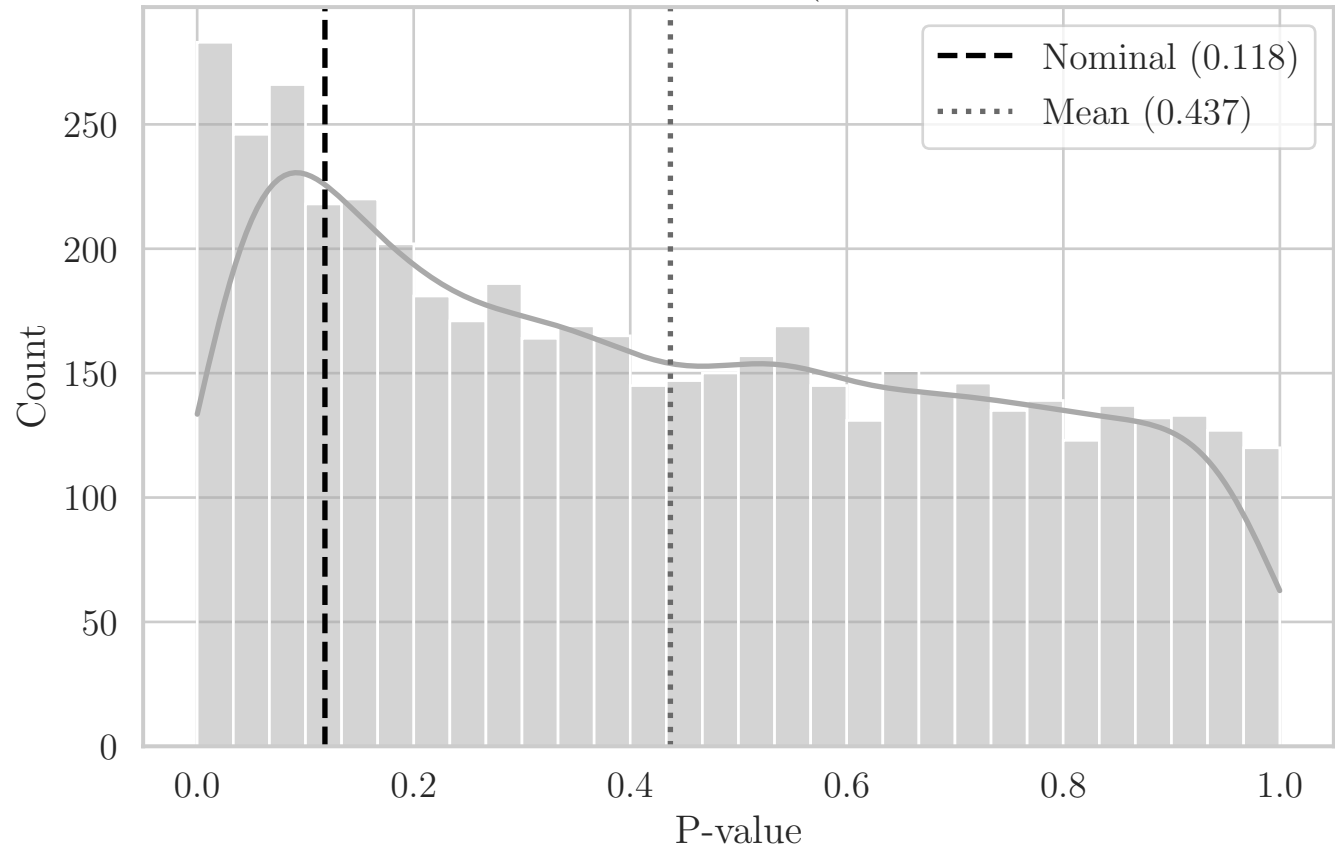
MC Distribution of P-values for ST Distance (Aggregated Top-Right Quadrant YZ)
