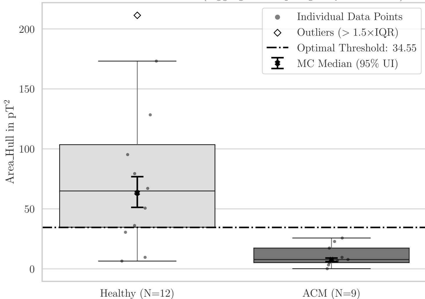
Box Plot for T Area_Hull (Aggregated Top-Right Quadrant YZ)
