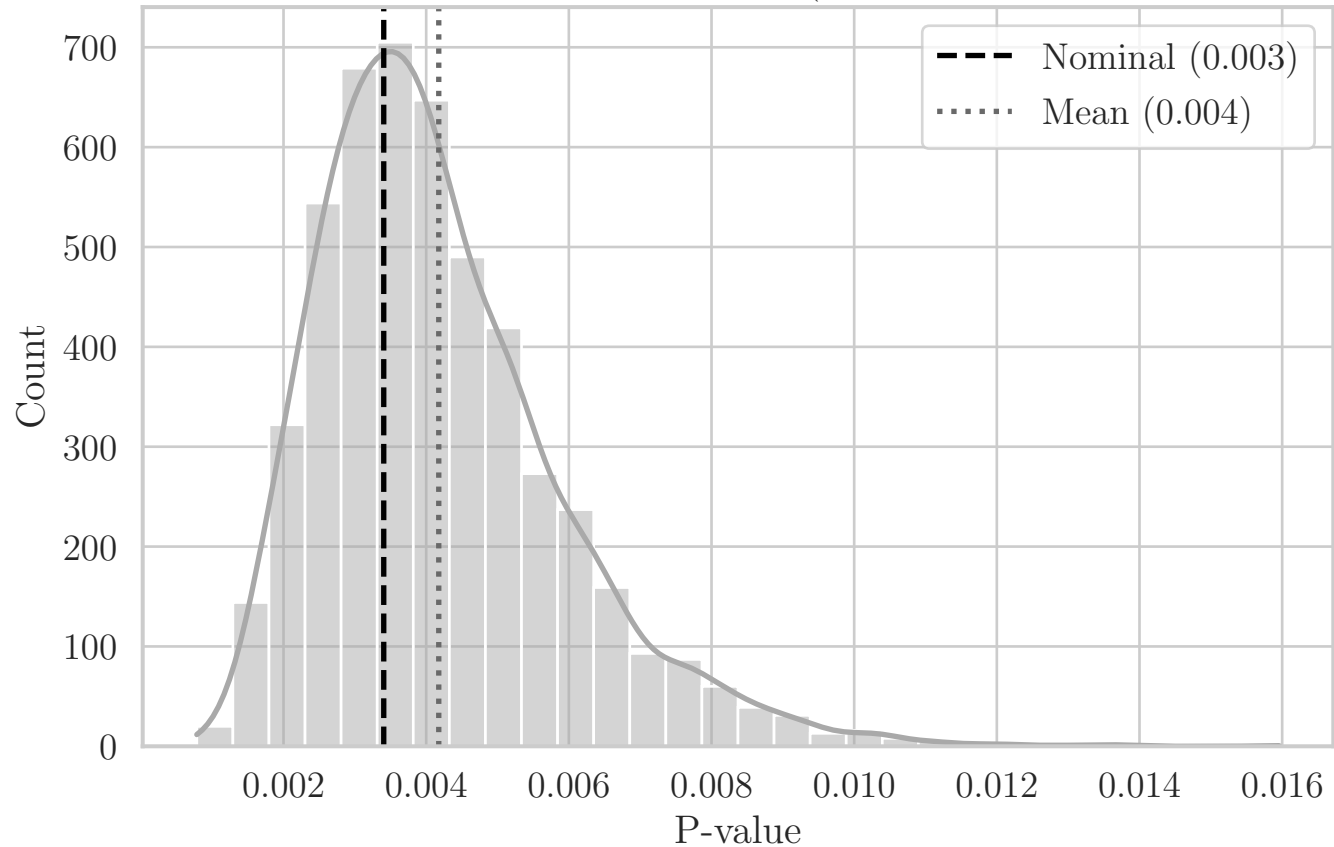
MC Distribution of P-values for T Area_Hull (Aggregated Top-Right Quadrant YZ)
