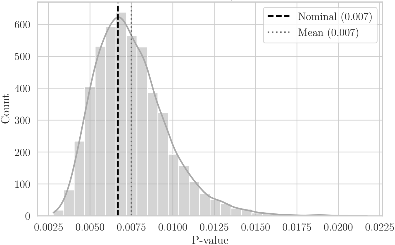
MC Distribution of P-values for T Area_Net (Aggregated Top-Right Quadrant YZ)
