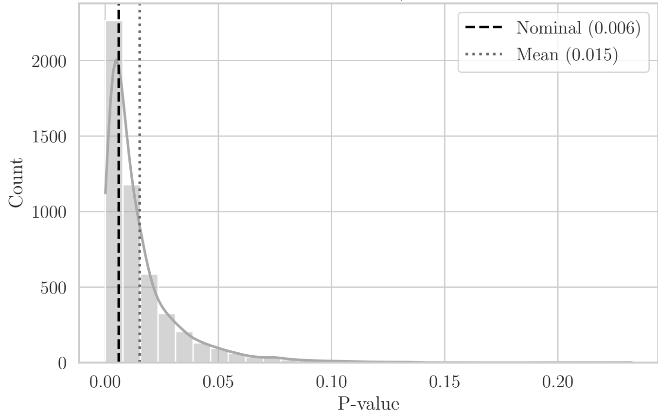
MC Distribution of P-values for T Distance (Aggregated Top-Right Quadrant YZ)
