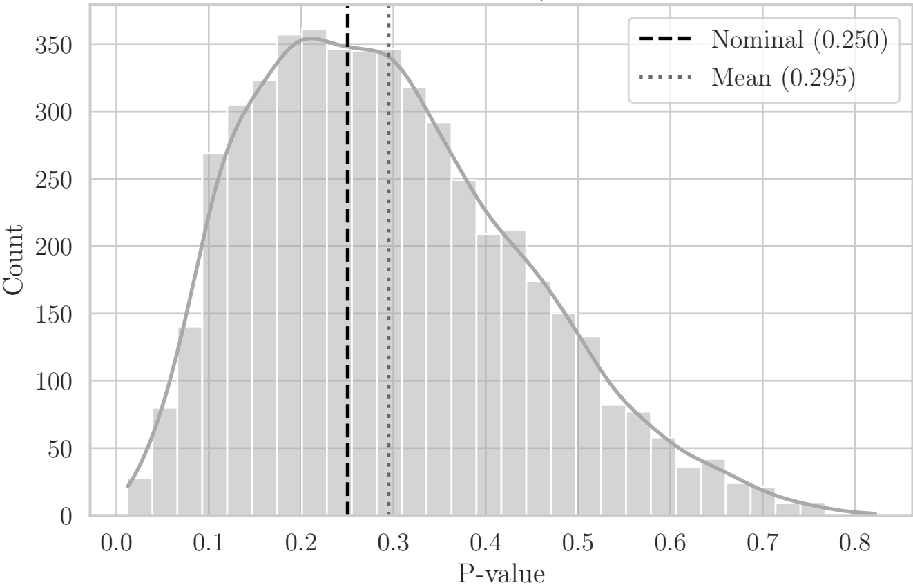
MC Distribution of P-values for T Solidity (Aggregated Top-Right Quadrant YZ)
