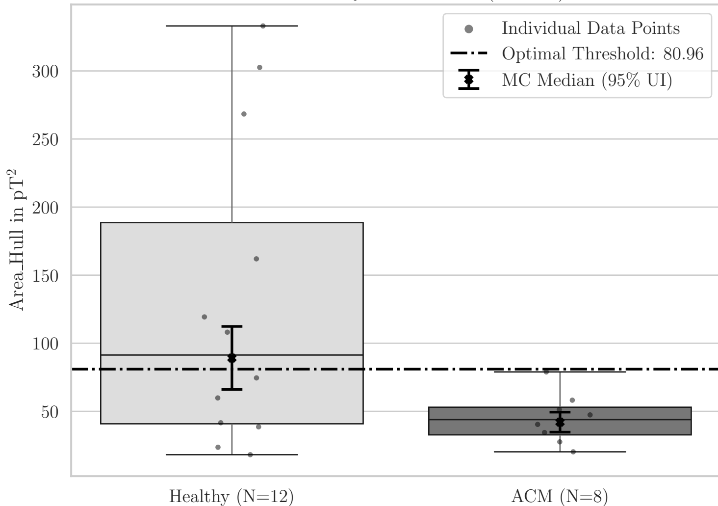
Box Plot for QRS Area_Hull (YP YZ)
