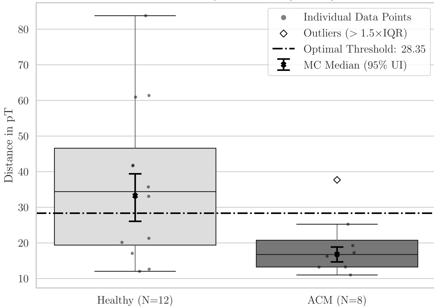
Box Plot for QRS Distance (YP YZ)
