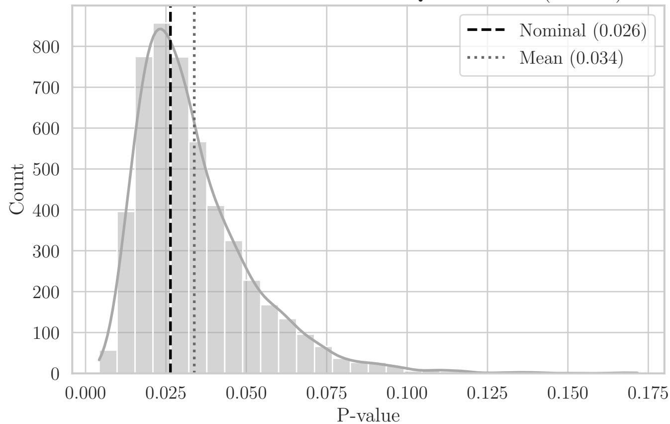
MC Distribution of P-values for QRS Distance (YP YZ)
