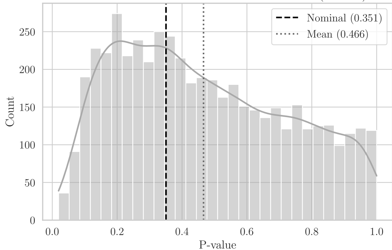
MC Distribution of P-values for ST Area_Hull (YP YZ)
