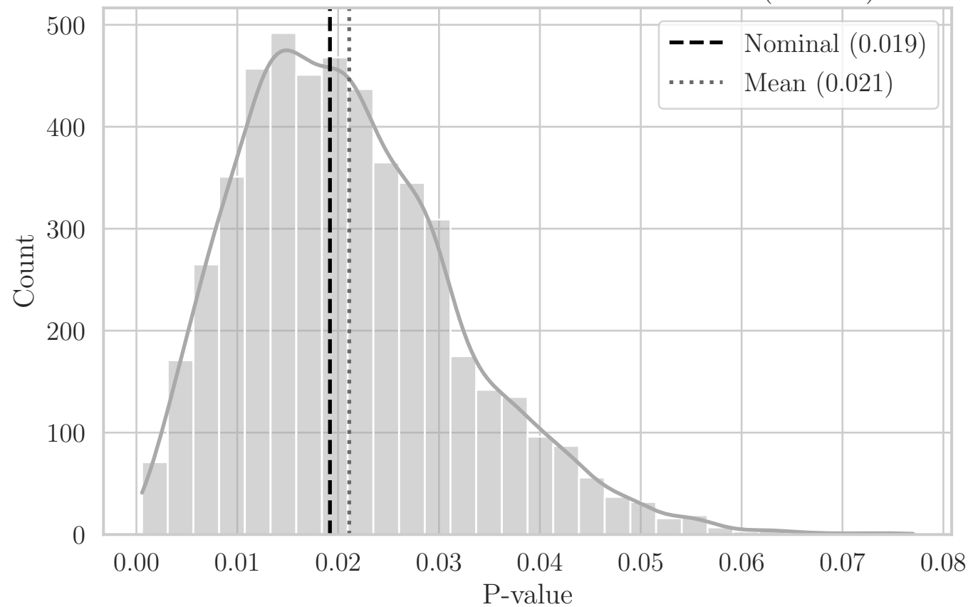
MC Distribution of P-values for T Area_Net (YP YZ)
