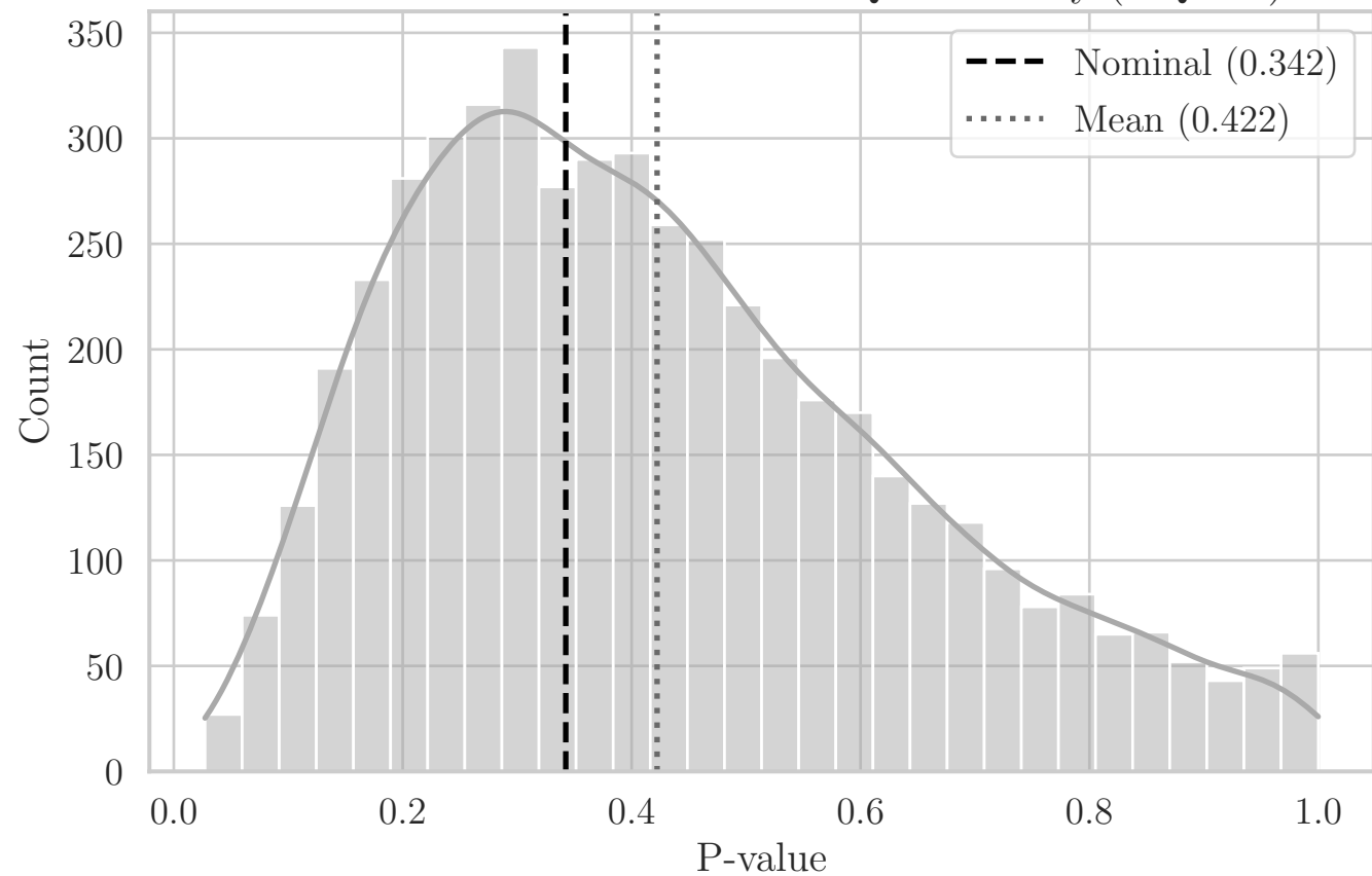
MC Distribution of P-values for QRS Solidity (YQ XY)
