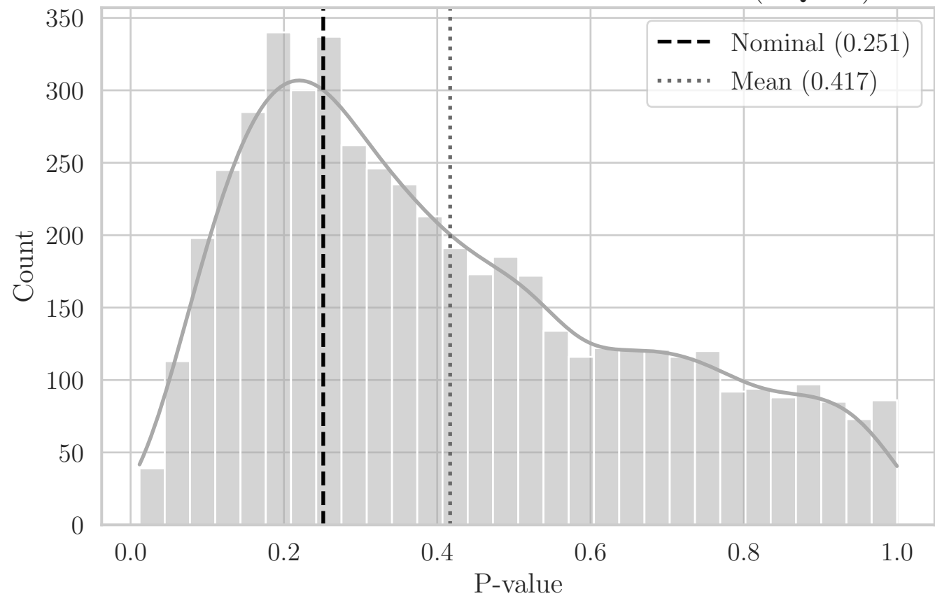
MC Distribution of P-values for ST Area_Net (YQ XY)
