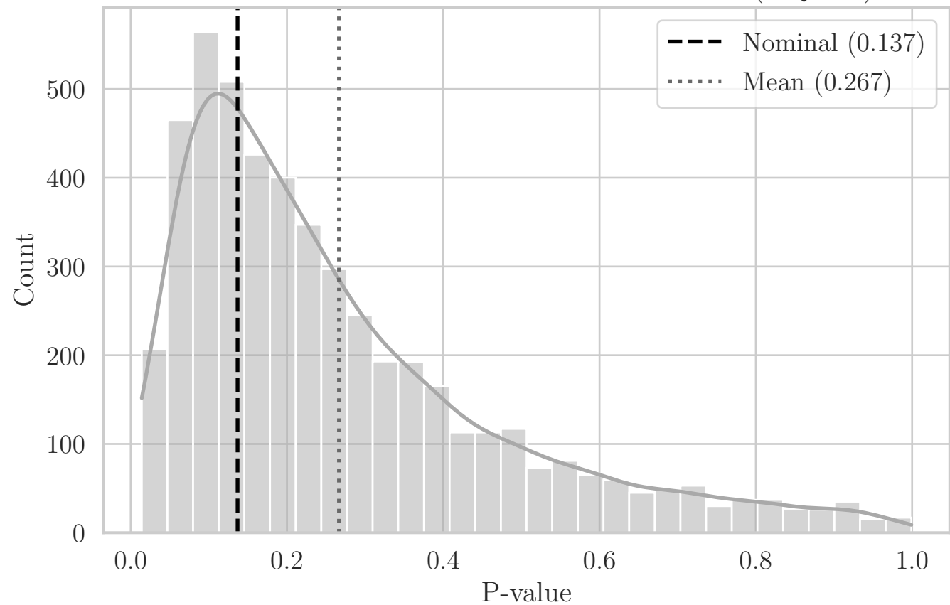
MC Distribution of P-values for T Distance (YQ XY)
