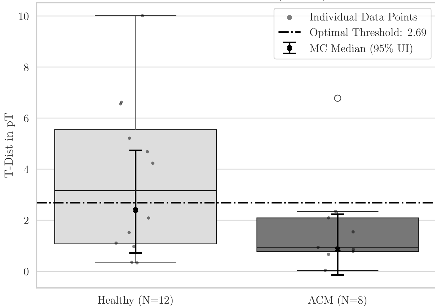
Box Plot for ST T-Dist (EY XY)
