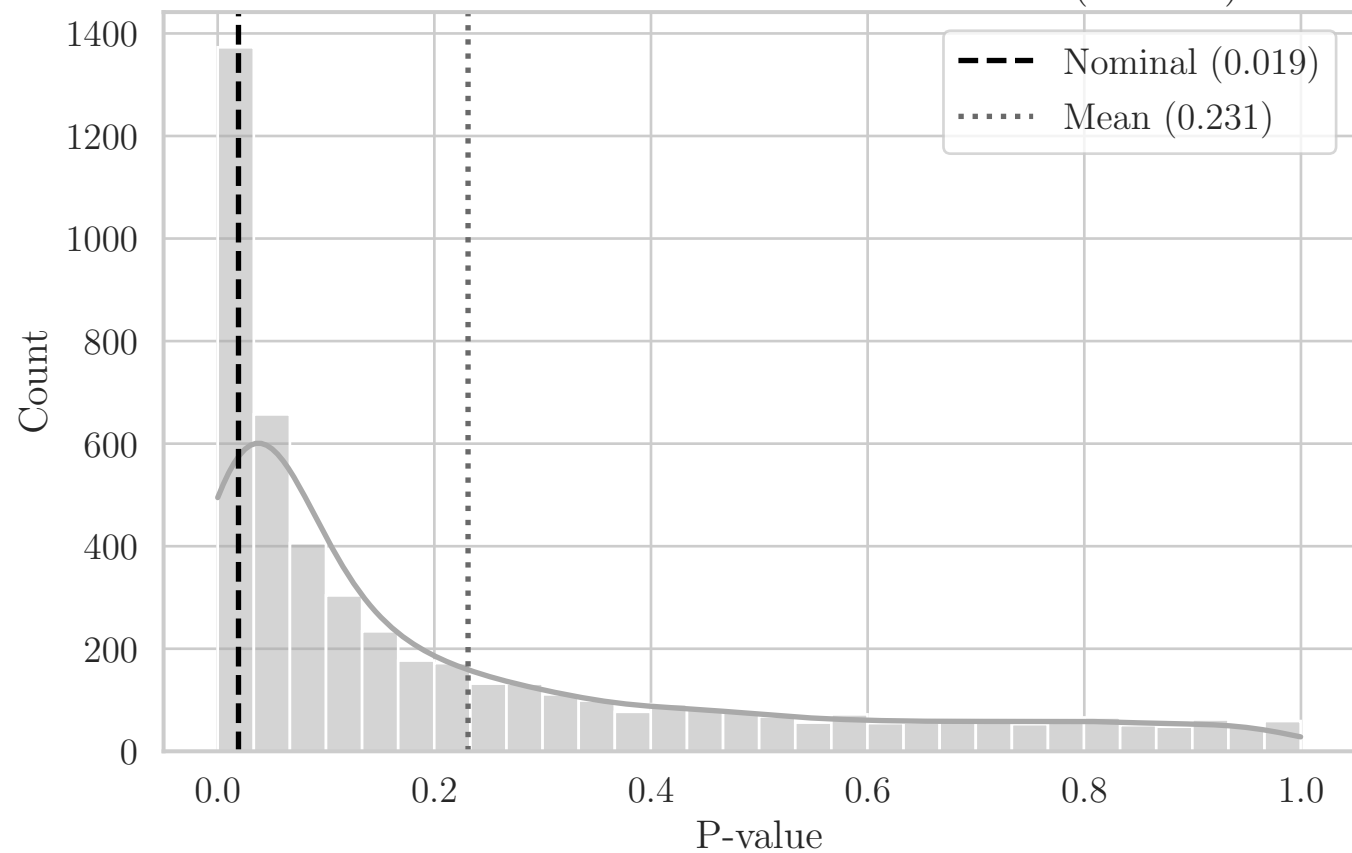
MC Distribution of P-values for ST T-Dist (EY XY)
