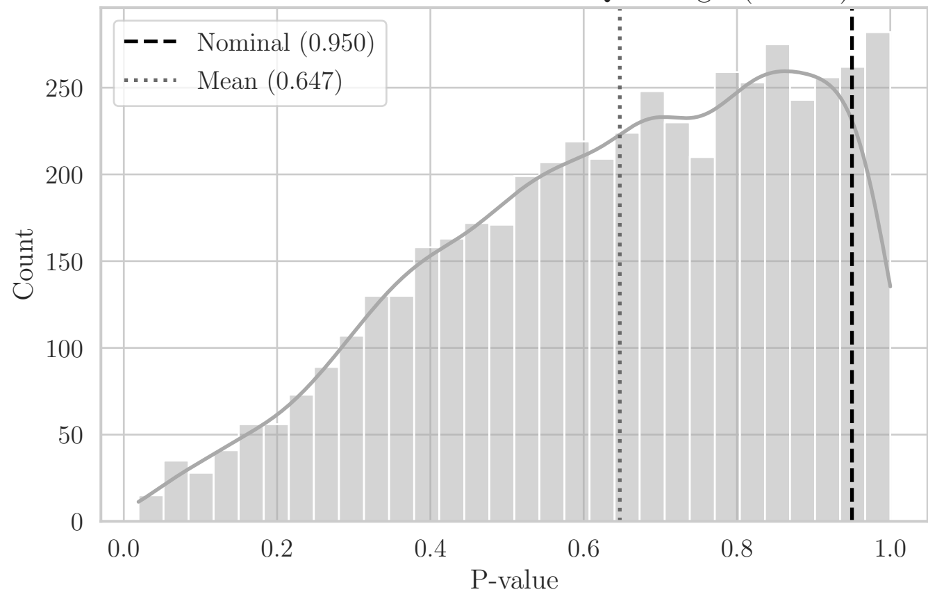
MC Distribution of P-values for QRS Angle (F2 XY)
